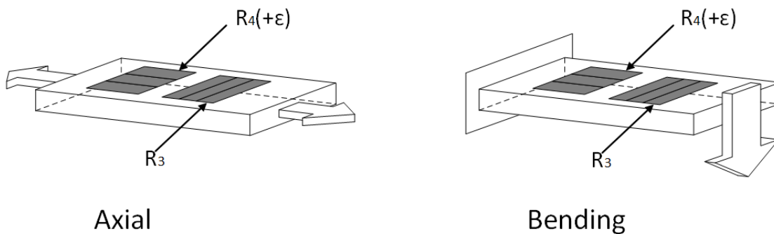
Figure 19 Quarter-Bridge Type II Measuring Axial and Bending Strain
