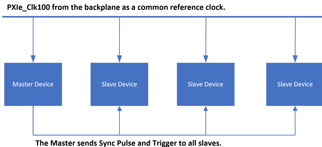
Figure 52 Multi-device Sync Topology
