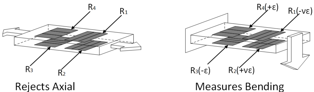
Figure 27 Full-Bridge Type II Rejecting Axial and Measuring Bending Strain
