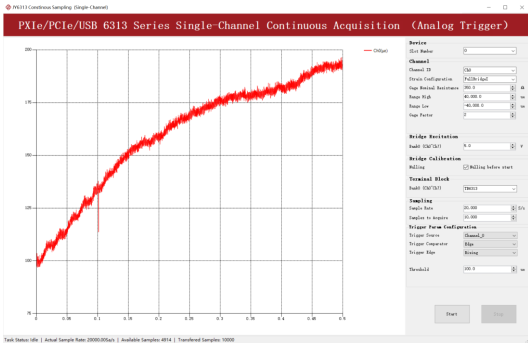
Figure 46 Acquisition result of Analog Trigger
