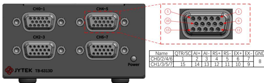
Figure 12 The front of TB-6313D
