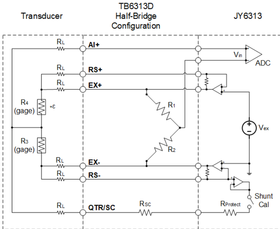
Figure 20 Quarter-Bridge Type II Circuit Diagram
