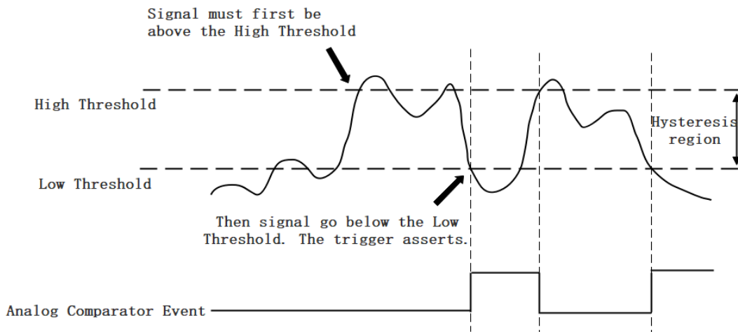
Figure 42 Hysteresis with Falling Slope Trigger
