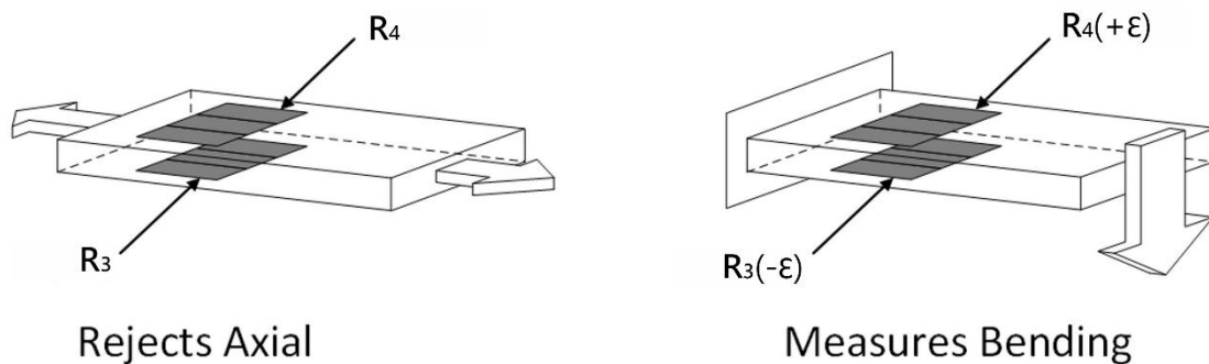
Figure 23 Half-Bridge Type II Rejecting Axial and Measuring Bending Strain
