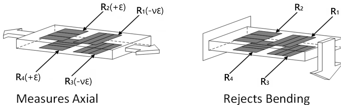
Figure 29 Full-Bridge Type III Measuring Axial and Rejecting Bending Strain
