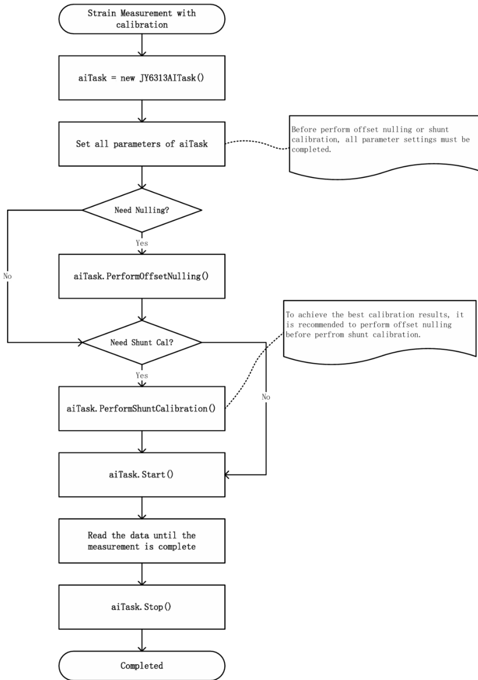
Figure 36 Bridge calibration process
