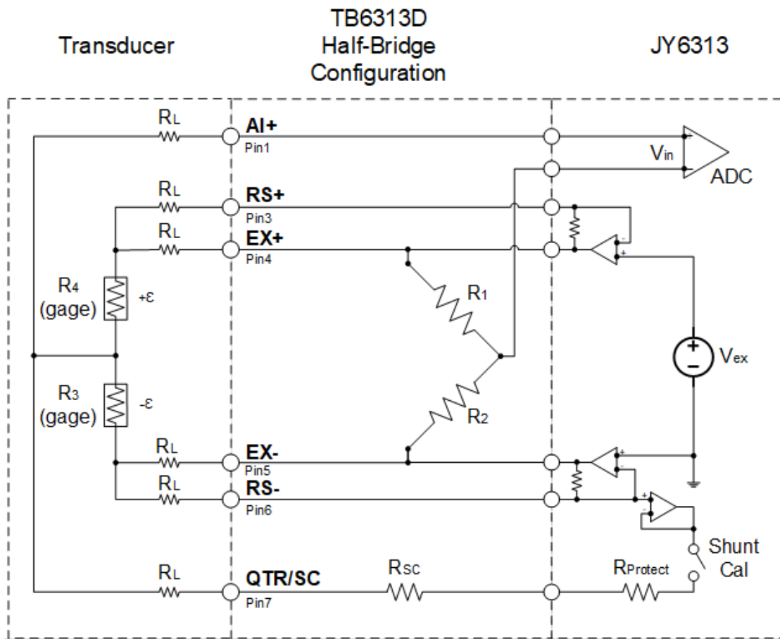
Figure 24 Half-Bridge Type II Circuit Diagram
