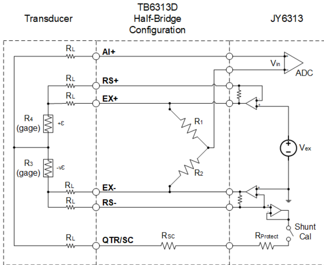
Figure 22 Half-Bridge Type I Circuit Diagram
