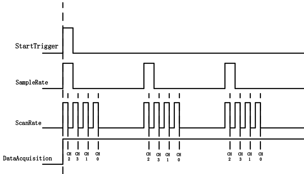
Figure 49 Start Trigger
