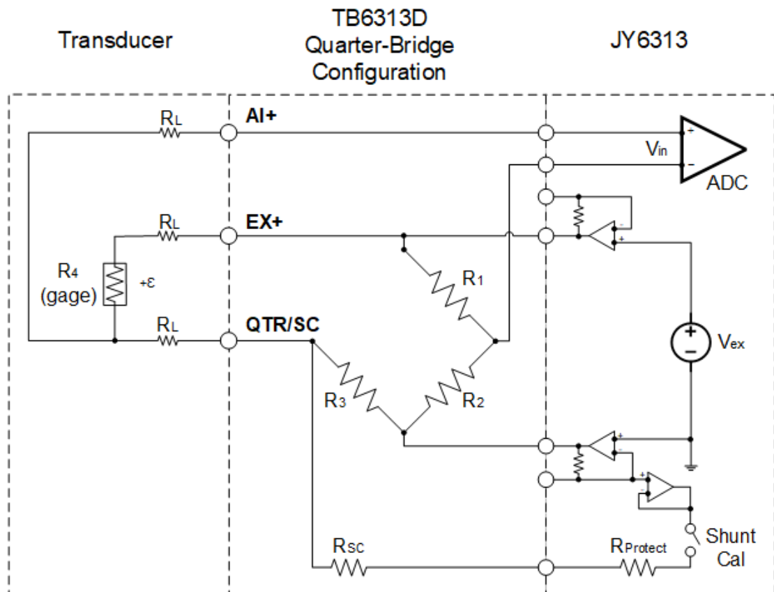
Figure 18 Quarter-Bridge Type I Circuit Diagram
