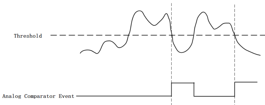
Figure 40 Falling Slope Trigger
