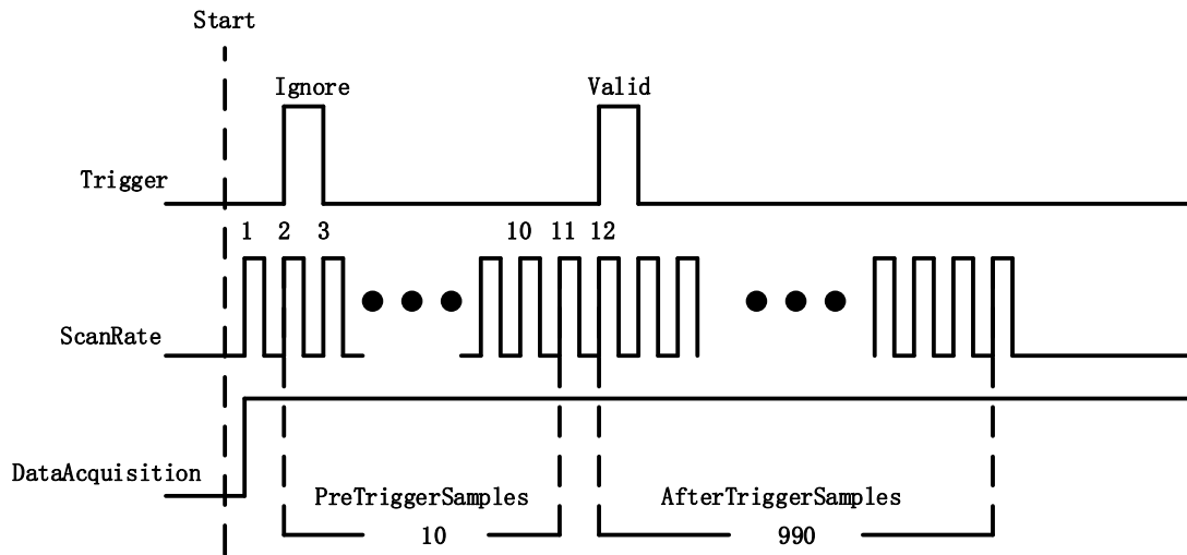
Figure 50 Reference Trigger
