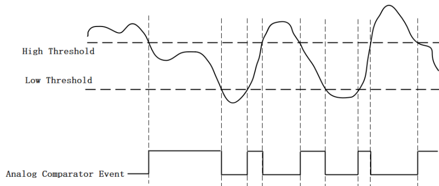
Figure 43 Entering Window Trigger
