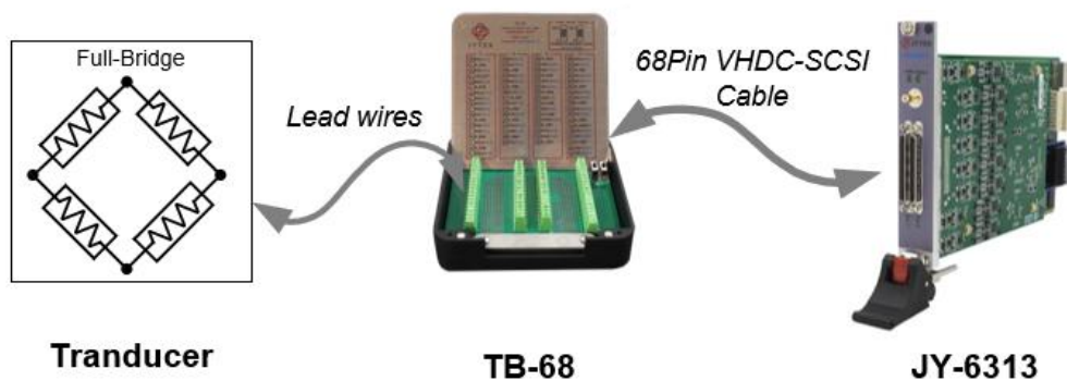
Figure 16 Connecting via TB-68(Only for Full-Bridge)
