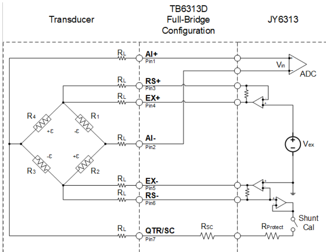
Figure 26 Full-Bridge Type I Circuit Diagram
