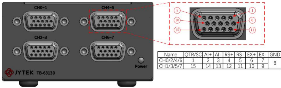
Figure 3 The front of TB-6313D
