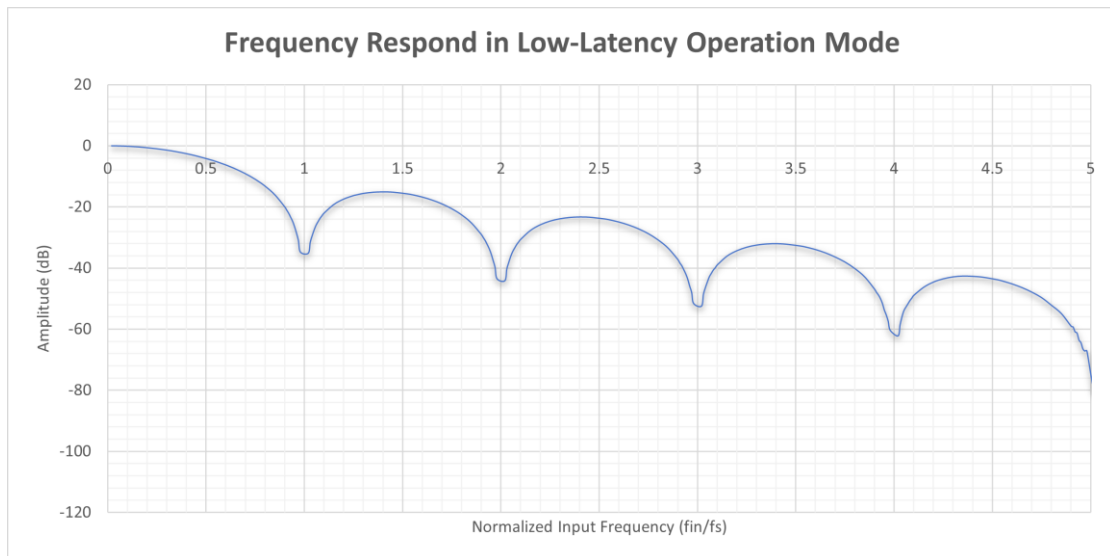
Figure 35 Frequency Respond (OperationMode = LowLatency)
