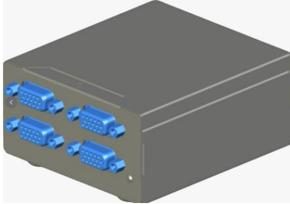
Figure 11 .Each TB-6313D can provide 8 transducer channels, Ch0 to Ch7.
