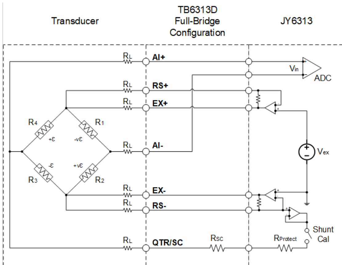
Figure 28 Full-Bridge Type II Circuit Diagram
