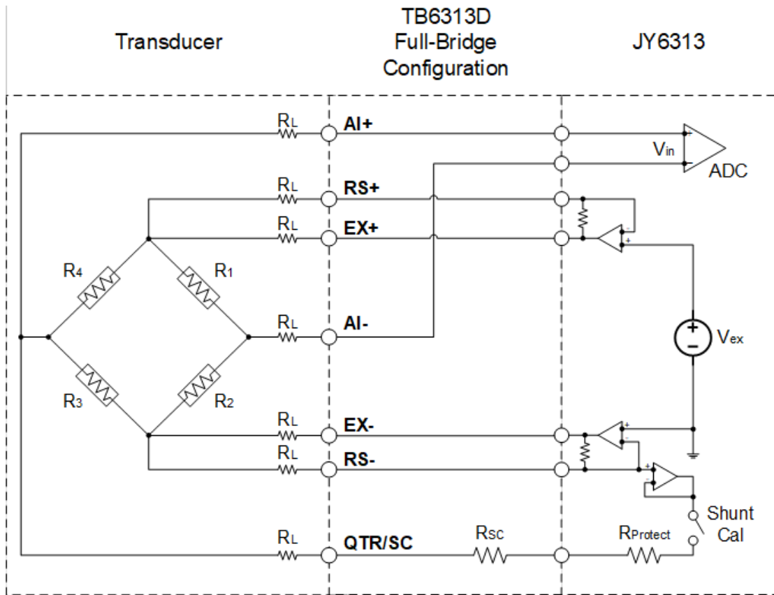
Figure 31 Full-Bridge with TB-6313D Circuit Diagram
