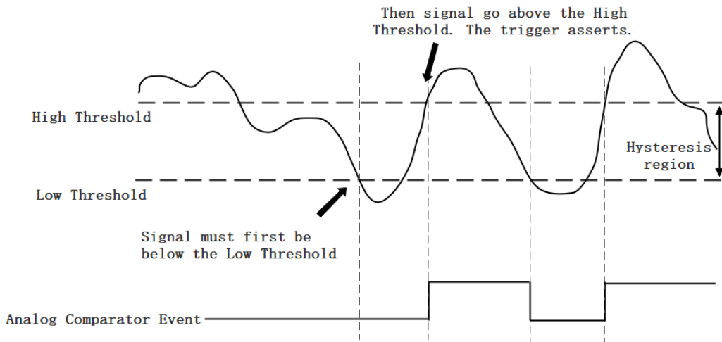
Figure 41 Hysteresis with Rising Slope Trigger
