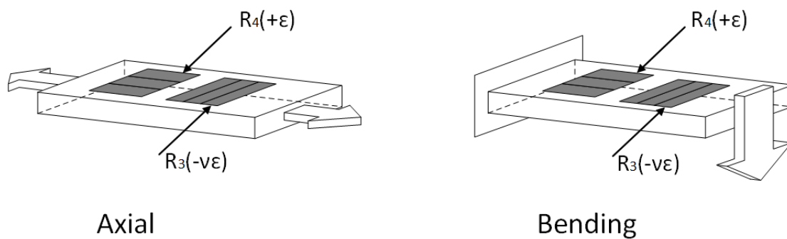
Figure 21 Half-Bridge Type I Measuring Axial and Bending Strain
