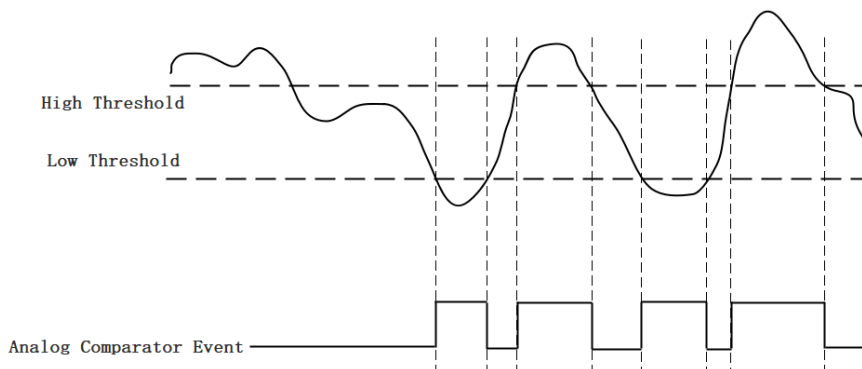
Figure 44 Leaving Window Trigger
