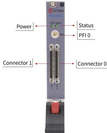
Figure 2 JY-6313 Front Panel
