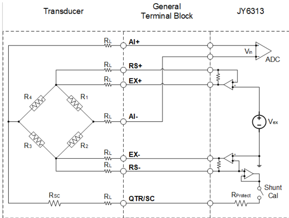
Figure 32 Full-Bridge with General Terminal Block Circuit Diagram
