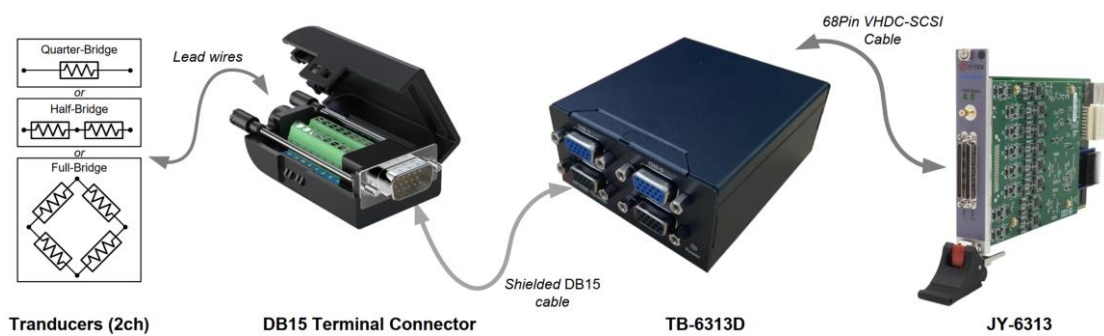
Figure 4 The front of TB-6313D
