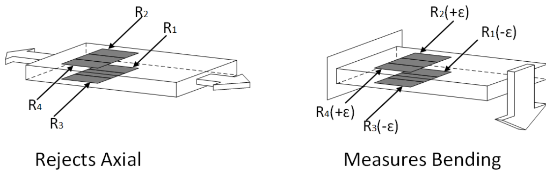
Figure 25 Full-Bridge Type I Rejecting Axial and Measuring Bending Strain
