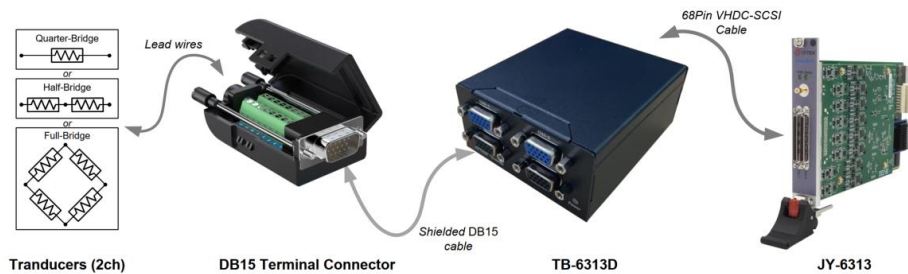
Figure 14 Connecting via TB-6313D
