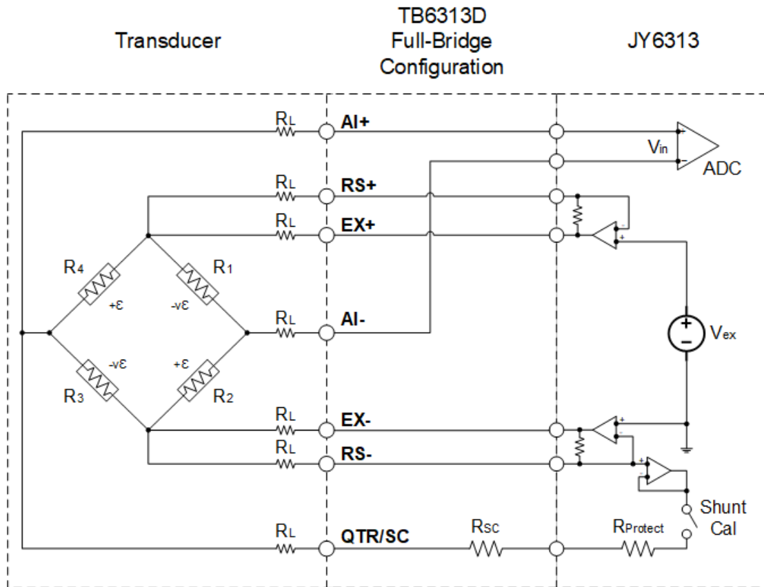
Figure 30 Full-Bridge Type III Circuit Diagram
