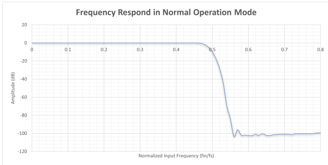
Figure 34 Frequency Response (OperationMode=Normal)
