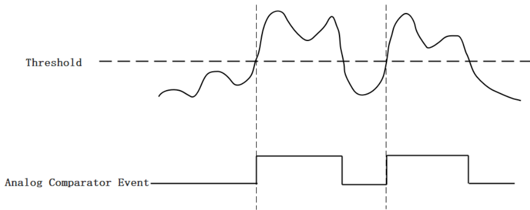
Figure 39 Rising Slope Trigger
