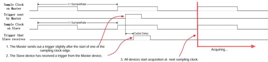
Figure 57 Master sends trigger to slave
